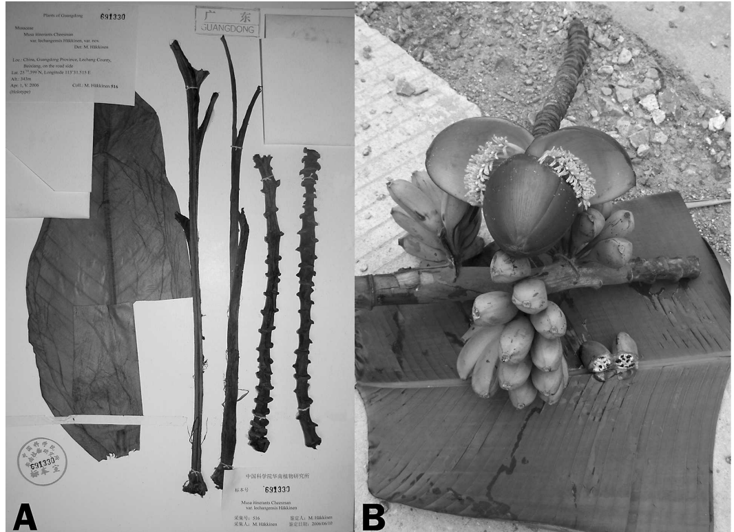
Figure 4. —A. Musa itinerans var. lechangensis Häkkinen. Holotype M. Häkkinen 516, IBSC. —B. Inflorescence and leaf part of variety lechangensis . Photos by Xiangying Wen from IBSC (A), and M. Häkkinen from Guangdong (B).
